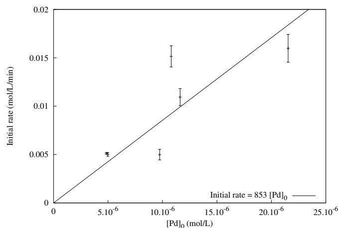
Figure 2. Effect of the initial concentration of Pd on the initial reaction rate. Conditions: 4-iodoacetophenone ( 0.05 \text{ mol/L} , 1 eq.), phenylboronic acid ( 0.06 \text{ mol/L} , 1.2 eq.), MeONa ( 0.075 \text{ mol/L} , 1.5 eq.), Pd from 5 \cdot 10^{-6} to 2.2 \cdot 10^{-5} \text{ mol/L} , ethanol ( 20 \text{ mL} ), and 60^\circ\text{C} .
