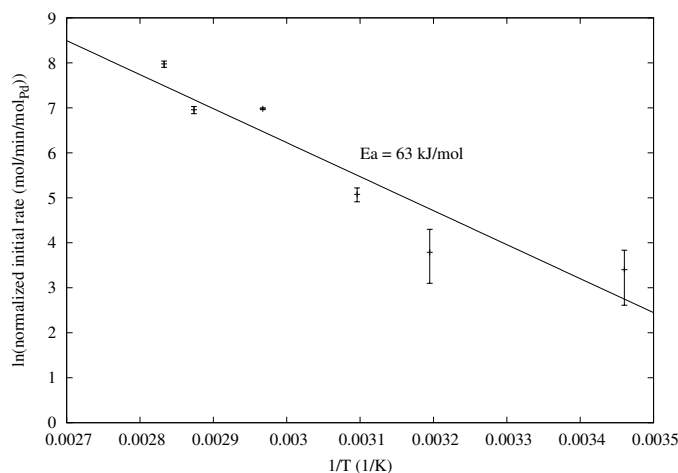
Figure 1. Arrhenius plot of Suzuki coupling of 4-iodoacetophenone and phenylboronic acid. The initial rates are normalized by the mass of Pd. Conditions: 4-iodoacetophenone ( 0.05 \text{ mol/L} , 1 eq.), phenylboronic acid ( 0.06 \text{ mol/L} , 1.2 eq.), MeONa ( 0.075 \text{ mol/L} , 1.5 eq.), Pd ( 5 \cdot 10^{-6} \text{ mol/L} ), and ethanol ( 20 \text{ mL} ).
