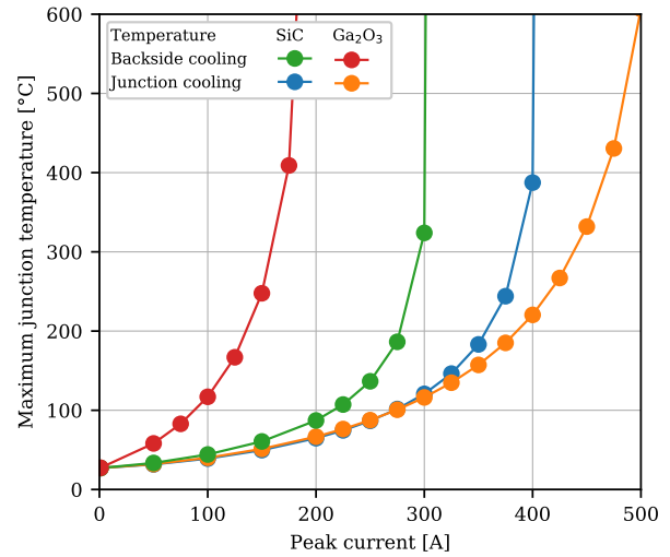
Fig. 9. Maximum temperature reached during a surge event as a function of the peak current, for 400 \mu\text{m} -thick SiC and \beta\text{-Ga}_2\text{O}_3 diodes.
