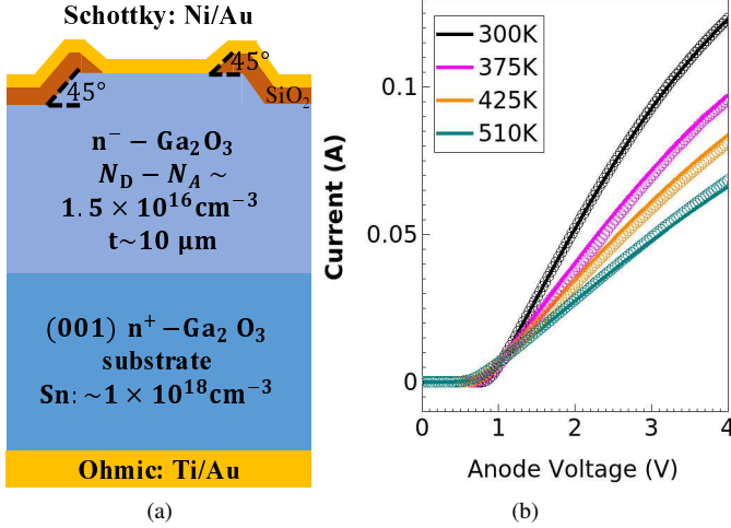
Fig. 1. (a) Structure of the fabricated \beta -Ga 2 O 3 Schottky barrier diodes. (b) Calibration of the TCAD simulation model: experimental (lines) and TCAD simulated (markers) IV curves at different temperatures.
