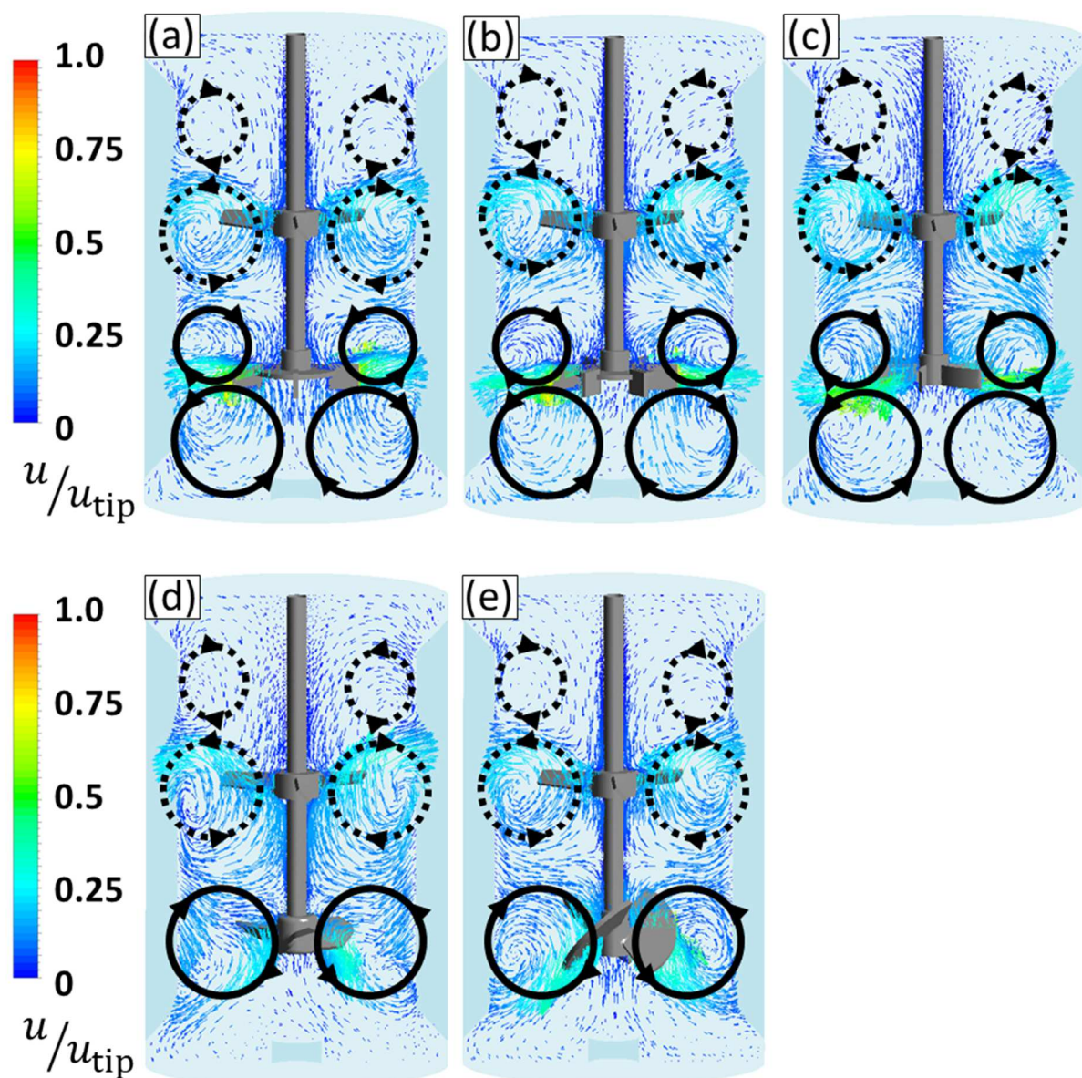
314 315 Fig. 4: Normalized liquid velocity vectors profiles at 500 rpm for: (a) the RT4B-A310 configuration; (b)
