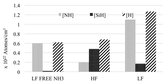
Fig. 2. Quantification of [Si-H], [N-H] and [H] from infra-red spectra of LF, HF and LF Free NH 3 samples.
