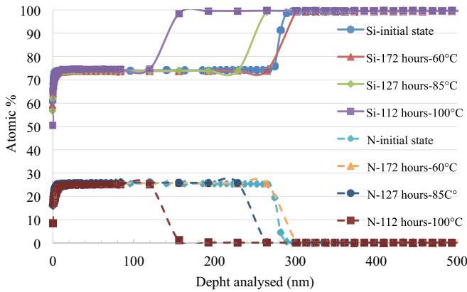
Fig. 5. Composition of the layer as a function of the analyzed depth obtained before and after dissolution of the HF sample soaked in water at initial state up to 100 °C for different durations. These data are deduced from XPS measurements.
