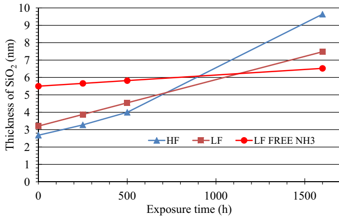
Fig. 3. Silicon oxide thickness as a function of exposure time at 85 °C/85% RH.
