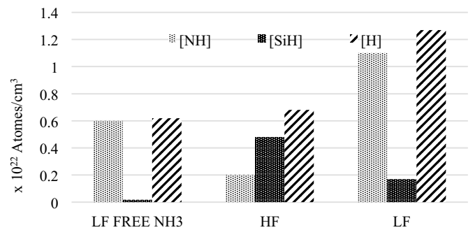
Fig. 2. Quantification of [Si-H], [N-H] and [H] from infra-red spectra of LF, HF and LF Free NH 3 samples.
