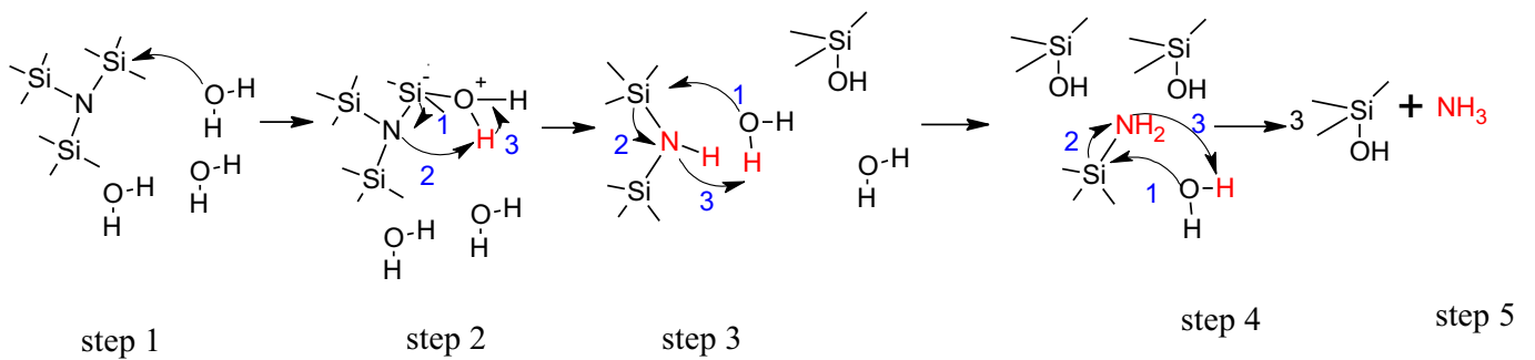
Fig. 6. Detailed chemical mechanism between water and \text{Si}_3\text{N}_4 from the equation 2 leading to the dissolution of the layer.
