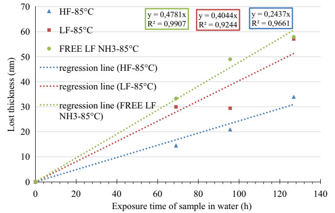
Fig. 4. Lost thicknesses of LF (red), HF (blue) and LF Free NH 3 (green) samples measured by SE as a function of the exposure time of sample in water at 85 °C.
