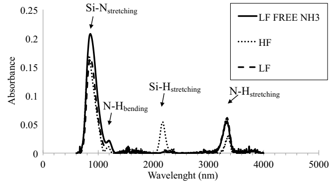
Fig. 1. Absorbance infra-red spectra of LF, HF and LF Free NH 3 samples.
