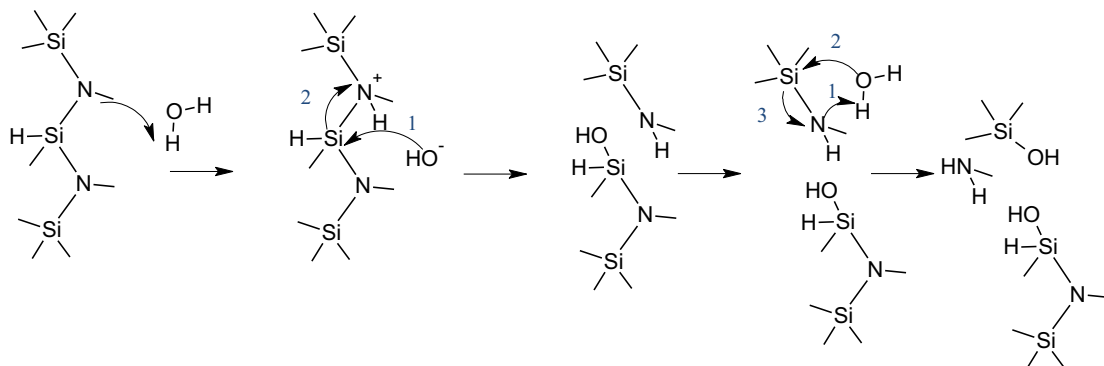
Fig. 7. The chemical mechanism between water and \text{Si}_6\text{N}_4\text{yHz} silicon rich structure (Si-H rich structure).
