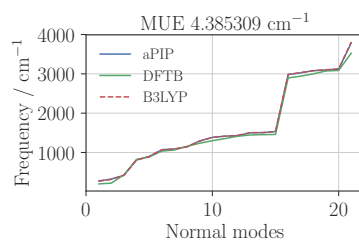
Figure S70: Normal Modes for Ethanol
