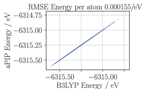
Figure S62: Comparison between the QM and PIP energies for Benzene
