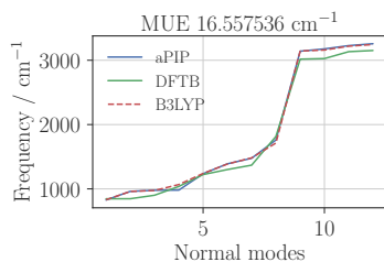
Figure S52: Normal Modes for Ethene
