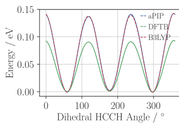
Figure S38: Dihedrals for Propane
