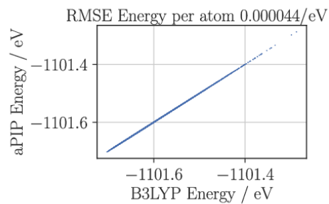
Figure S27: Comparison between the QM and PIP energies for Methane
