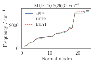
Figure S41: Normal Modes for Butadiene
