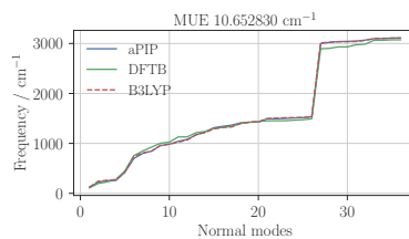
Figure S6: Normal Modes for Butane
