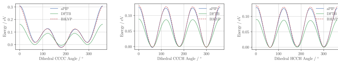
Figure S9: Dihedrals for Butane
