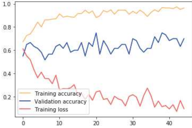
Fig. 5: Proposed method accuracy graph and loss graph for training and validation sets after each epoch.
