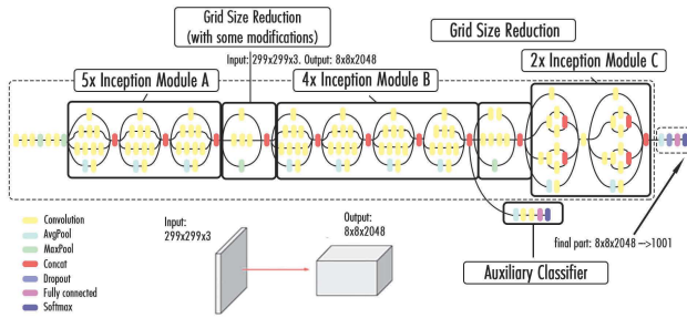
Fig. 4: Architecture of the Inceptionv3 model.
