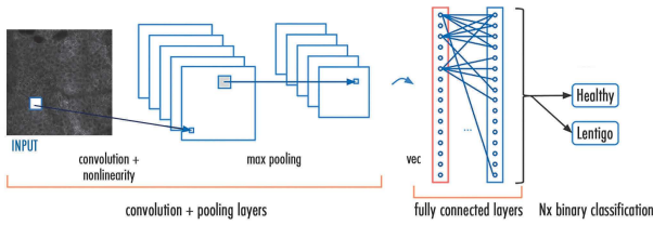
Fig. 2: The CNN architecture model.
