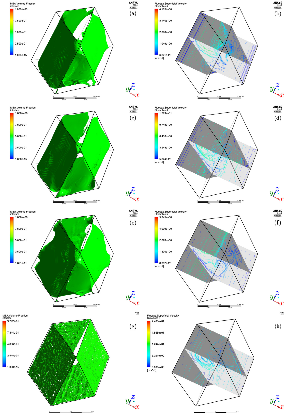
Fig. 14. Interface (left panel) and gas-streamline pattern (right panel) for different Re_G , angles and liquid loads: (a-b) Re_G = 270 , \beta = 45^\circ , B = 130 \text{ m}^3/\text{m}^2/\text{h} ; (c-d) Re_G = 1365 , \beta = 45^\circ , B = 130 \text{ m}^3/\text{m}^2/\text{h} ; (e-f) Re_G = 270 , \beta = 30^\circ , B = 130 \text{ m}^3/\text{m}^2/\text{h} ; (g-h) Re_G = 1652 , \beta = 45^\circ , B = 1.3 \text{ m}^3/\text{m}^2/\text{h} . The interface is computed as the iso-surface of volume fraction at 0.5. Counter-current channel: y-direction; co-current channel: z-direction.
