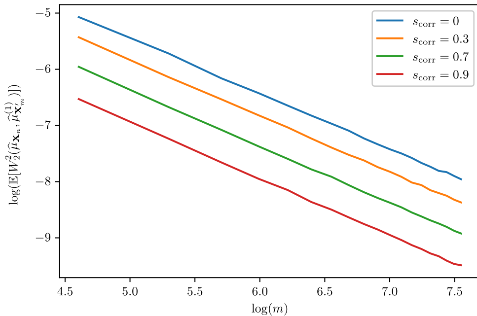
FIGURE 3. Evolution of \mathbb{E}[W_2^2(\widehat{\mu}_{\mathbf{X}_n}, \widehat{\mu}_{\mathbf{X}'_m}^{(1)})] with respect to m , for various values of s_{\text{corr}} . For each value of m and s_{\text{corr}} , the quantity W_2^2(\widehat{\mu}_{\mathbf{X}_n}, \widehat{\mu}_{\mathbf{X}'_m}^{(1)}) is computed (with n = 100 ) thanks to the formula (9), and its expectation is estimated through Monte Carlo average over 700 replications. The theoretical rate of m^{-q/d} = m^{-1} is attained for each experiment.
