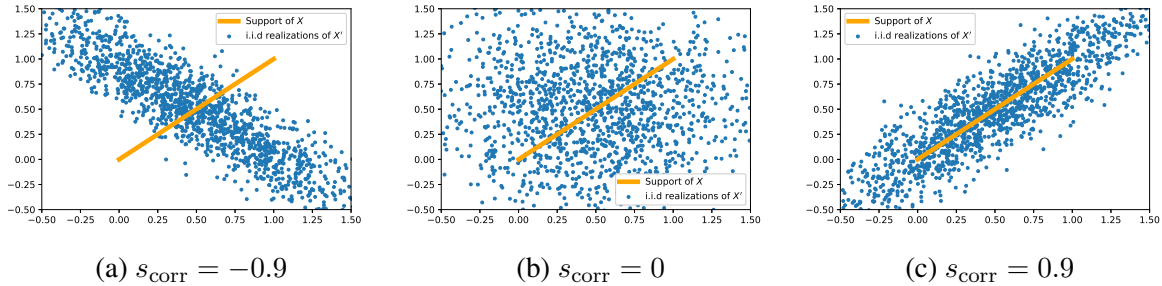
FIGURE 1. Plot of the support of X and 1500 i.i.d. realizations of X' for different values of s_{\text{corr}} .
