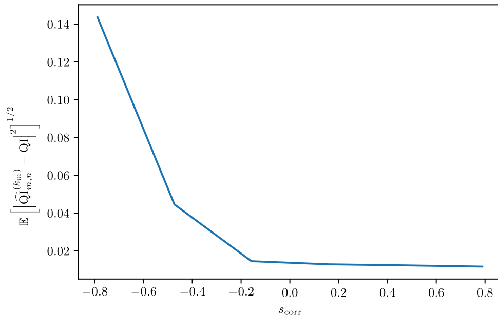
FIGURE 4. Estimation of the L^2 error with respect to s_{\text{corr}} for n = m = 900 and k_m = 4 , averaged on 2000 replications.
