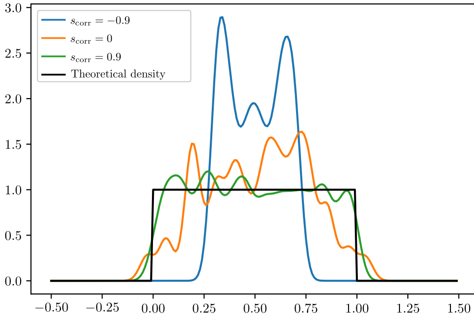
FIGURE 2. Trace of a kernel smoothing of \widehat{\mu}_{\mathbf{X}'_m}^{(1)} on the segment \{(u, u), u \in [0, 1]\} for different values of s_{\text{corr}} .
