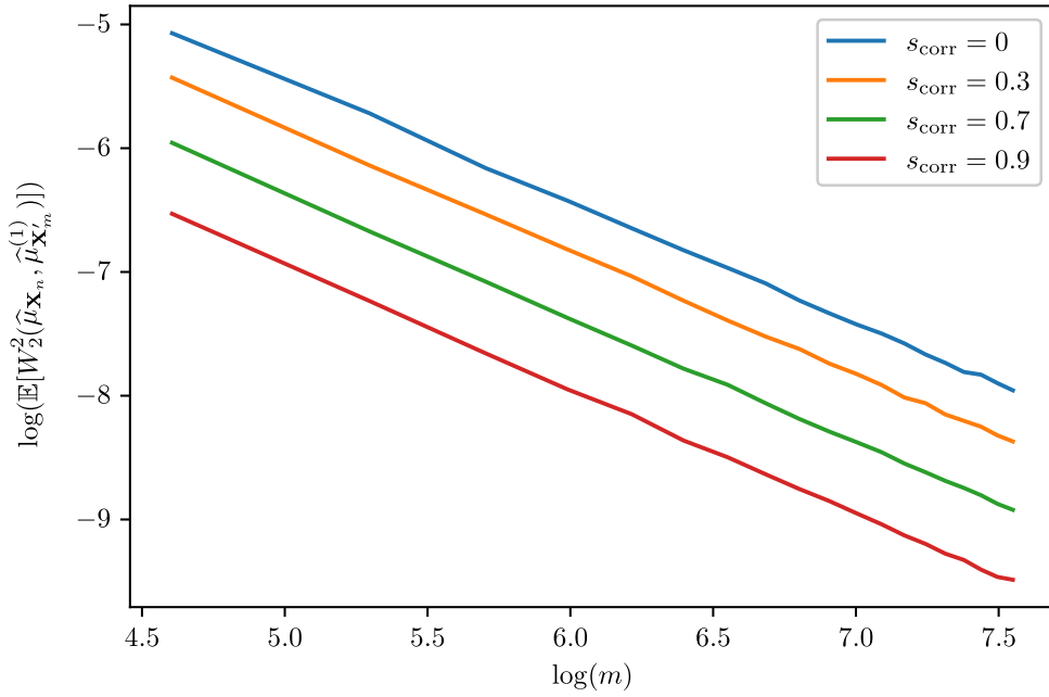
FIGURE 3. Evolution of \mathbb{E}[W_2^2(\hat{\mu}_{\mathbf{X}_n}, \hat{\mu}_{\mathbf{X}'_m}^{(1)})] with respect to m , for various values of s_{\text{corr}} . For each value of m and s_{\text{corr}} , the quantity W_2^2(\hat{\mu}_{\mathbf{X}_n}, \hat{\mu}_{\mathbf{X}'_m}^{(1)}) is computed (with n = 100 ) thanks to the formula (9), and its expectation is estimated through Monte Carlo average over 700 replications. The theoretical rate of m^{-q/d} = m^{-1} is attained for each experiment.
