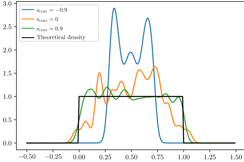
FIGURE 2. Trace of a kernel smoothing of \hat{\mu}_{\mathbf{X}'_m}^{(1)} on the segment \{(u, u), u \in [0, 1]\} for different values of s_{\text{corr}} .
