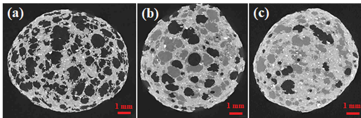
Fig. 3. Tomography images of fish feed pellets: (a) uncoated pellet, (b) coated pellet produced using a 299 mbars pressure in the pilot vacuum coater, and (c) coated pellet produced using a 151 mbars pressure in the pilot vacuum coater (55 Hz stirring speed and 45 % filling rate of the coater during vacuum coating).
