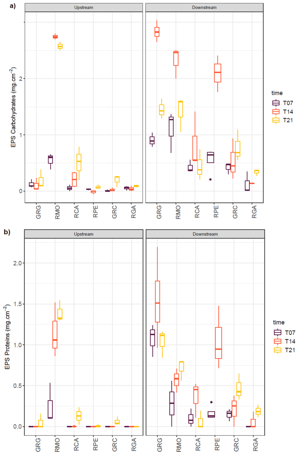
Figure 3. (a) Extracellular carbohydrates of upstream (left panel) and downstream (right panel) epilithic biofilms measured by colorimetry ( \text{mgEq Glucose}/\text{cm}^2 ). Sampling sites were ordered from the least polluted to the most polluted according to the order given in Fig. 1b for downstream sites, (b) extracellular proteins of upstream (left panel) and downstream (right panel) epilithic biofilms measured by colorimetry ( \text{mgEq BSA}/\text{cm}^2 ). Sampling sites were ordered from the least polluted to the most polluted according to the order given in Fig. 1b for downstream sites.
