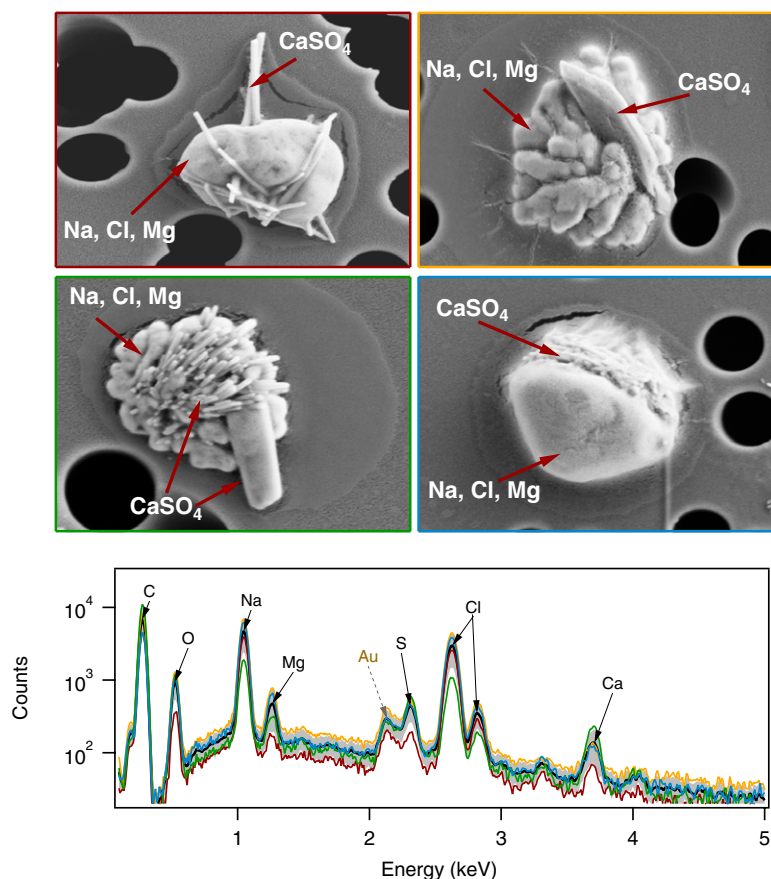
Fig. 7. SEM images of sea salt particles collected in the western Pacific Ocean. The four particles had similar X-ray spectra, shown below the images. The color of the frame of each SEM image corresponds to the color of the X-ray spectrum trace; the average of them is shown in black with the standard deviation shown as a shaded gray area. The black holes are 0.8 \mu\text{m} in diameter.
