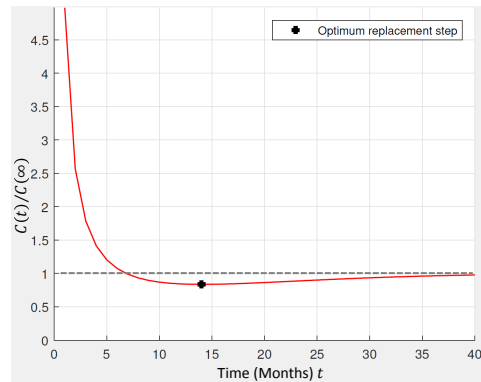
Fig. 5. Cost function associated to the cluster 1
