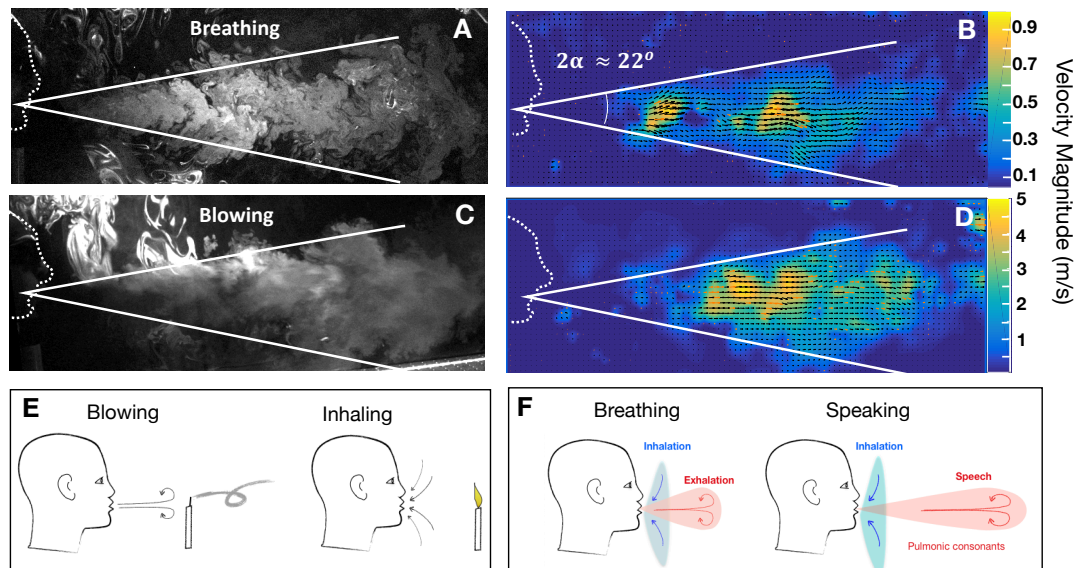
Fig. 1. Flow visualization snapshot of exhalation in a laboratory-generated fog and parallel to a laser sheet in two different breathing situations. (A) Calm breathing with (B) the corresponding flow speeds shown with the color code and arrows, and (C) a case of strong blowing with (D) the corresponding velocity field. Notice the much higher velocities associated with blowing. However, the flows in the two cases are qualitatively similar over a sufficiently long period of time of a few seconds and exhibit jet-like features. The field-of-view in all of the images is 1 meter. (E) Sketch of blowing out a candle (or not). (F) Sketch of the qualitative contrast between exhalation and inhalation for breathing and speaking.
