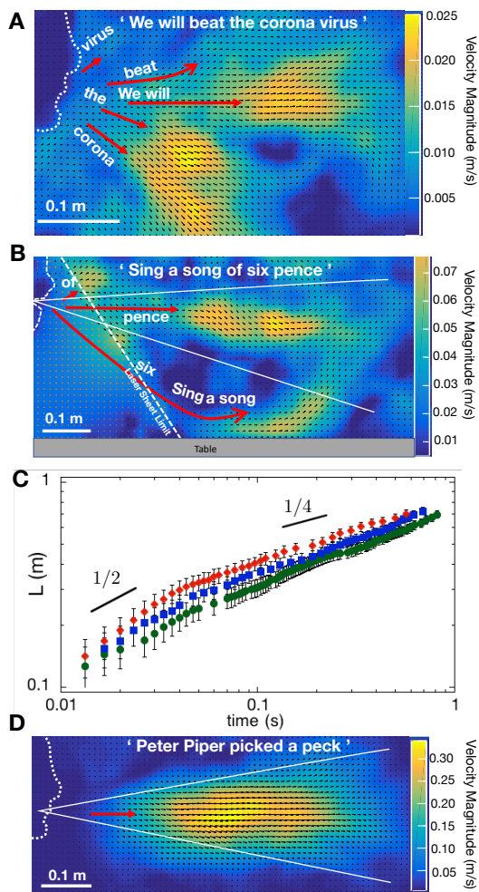
Fig. 2. Mean velocity field produced when speaking three different sentences. A color code illustrates the average speeds but note that single images of the magnitude of speeds are not representative of the true instantaneous velocities, which were estimated from the movies in the SI. (A) ‘We will beat the corona virus’, which is a mixture of vowels, fricatives and plosives. (B) ‘Sing a song of six pence’ (SSSP) (?), mainly composed of the fricative ‘S’ except the last word that starts with ‘P’. (C) The distance travelled by the extremity of the air puff as a function of time when saying ‘pence’ at the end of SSSP for three different runs. (D) ‘Peter Piper picked a peck’ (PPPP) (?), which is mainly composed of many plosives ‘P’.
