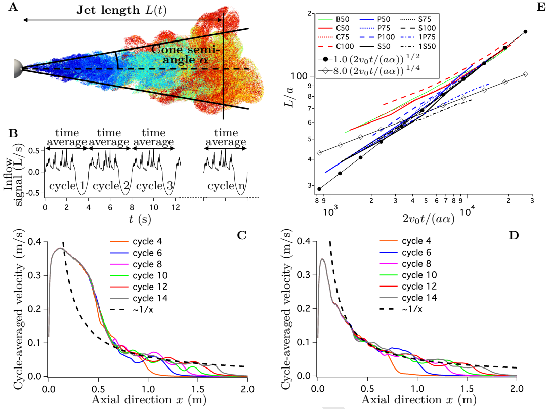
Fig. 5. Jet characteristics in the simulation of the breathing and speaking signals shown in Fig. ??A-D. (A) Example of calculation of jet length L and angle \alpha for S75, based on the emitted tracer particles color-coded here by residence time, as described in Fig. ??E-H. L(t) is such that 90% of the particles are located upstream of x = L at time t . The cone angle \alpha is calculated to enclose 90% of the particles is a cone passing through the mouth exit (radius is 1 cm at x = 0 ). This angle is verified to remain stable with time after the initial cycles. (B) Principle of the calculation of the cycle-averaged velocity fields presented in (C-D): The velocity is time-averaged independently over each cycle. (C-D) Progressive formation, along increasing cycles of exhalation and inhalation, of a turbulent jet-like velocity profile v(x) in the far field. Examples of cases C50 (C) and S50 (D): cycle-averaged axial velocity along the x axis from the mouth exit to 2.0 m downstream, for different cycles, extending to 14 cycles or 56 s. The black dashed line is the v(x) \propto 1/x scaling, plotted here as a guide for the eye, which is suggested by a model of a steady turbulent jet. (E) Evolution of the non-dimensional jet length L/a as a function of 2v_0t/(a\alpha) (see Eq. ??), with a \approx 1.22 cm the equivalent radius of the mouth exit and v_0 the average axial speed during exhalation for the different simulations. Two power laws are plotted as a guide for the eyes to assess the evolution of L with time. Raw data L(t) is plotted in Fig. S2.
