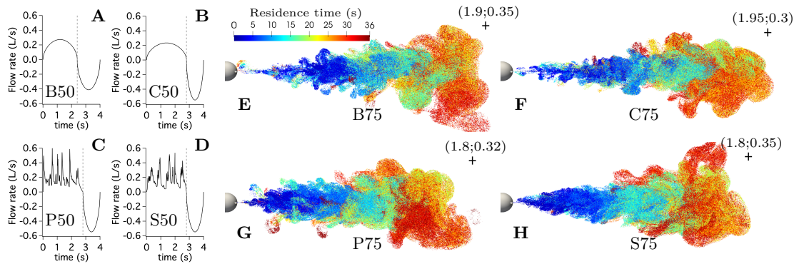
Fig. 4. Numerical simulations of periodic breathing versus speaking signals for cycles of 4.0 s. The jets issue from a sphere with an open elliptic orifice of semi-axes 1.0 cm and 1.5 cm. (A-D) volumetric flow rate signals for cases with 0.5 L per breath (hence the '50' in the labels), where the vertical dashed lines mark the separation between exhalation and inhalation. (A) Case B50 is a breathing-like signal with 2.4 s exhalation and 1.6 s inhalation. (C) Case P50 and (D) case S50 are speaking signals sampled from (?), and recorded during articulation of 'Peter Piper picked a peck' and 'Sing a song of six pence', respectively, with speaking time of 2.8 s and a 1.2 s inhalation. The P50 and S50 signals have been adjusted to 0.5 L per breath. (B) Case C50 is a calm signal of the same macroscopic characteristics as P50 and S50, but with a smooth signal similar to B50. Three series of simulations have been performed at different volumes per breath, i.e., 0.5 L, 0.75 L and 1.0 L per breath. For the simulation of 'Peter Piper picked a peck' for instance, the simulations at 0.75 L and 1.0 L per breath are referred to as P75 and P100, and are obtained by multiplying the input flow rate signal of P50 by 1.5 and 2.0, respectively. (E-H) Examples of jets obtained for cases B75, C75, P75 and S75 after 9 cycles (36 s), as visualized by perfect tracers issued from the mouth and color-coded by their residence time in the computational domain (dark blue tracers were exhaled during the last cycle). The scale is the same for all plots. For each case, a point marked by a '+' is positioned to indicate the axial and radial extent of the jet. The x and y coordinates of the point are reported as (x;y) in the figures (E-H).
