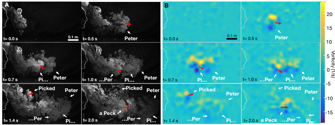
Fig. 3. Time evolution of the flow from a sentence, ‘Peter Piper picked a peck’ (PPPP), with many plosives, spoken parallel to a laser sheet. The speaker is indicated by the dotted curve to the left. to the (A) Flow visualization with the individual plosives identified. (B) Vorticity field with individual vortices clearly visible for each plosive ‘P’ pronounced in the sentence. Notice the interactions between the first vortices, as well as the different upward angle of the vortex produced when the syllable ‘Pi’ is pronounced in ‘picked’.
