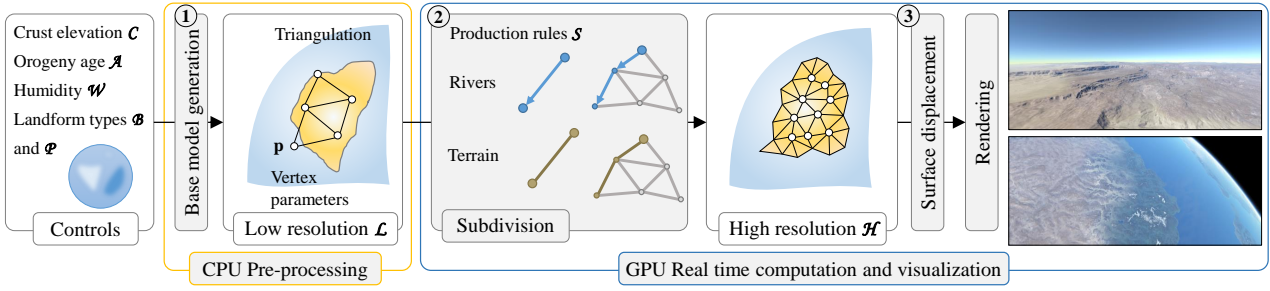
Fig. 3 Given several control maps \mathcal{M} defining the crust elevation \mathcal{C} , the orogeny age \mathcal{A} , the wetness \mathcal{W} and the landform type \mathcal{P} or \mathcal{B} , we synthesize an initial low-resolution model \mathcal{L} which is recursively amplified in real time by using subdivision rules to generate details.
