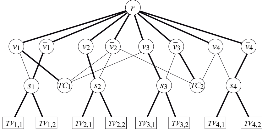
Figure 7: From 3-SAT 3 to CAP-STEINER-TREE.
