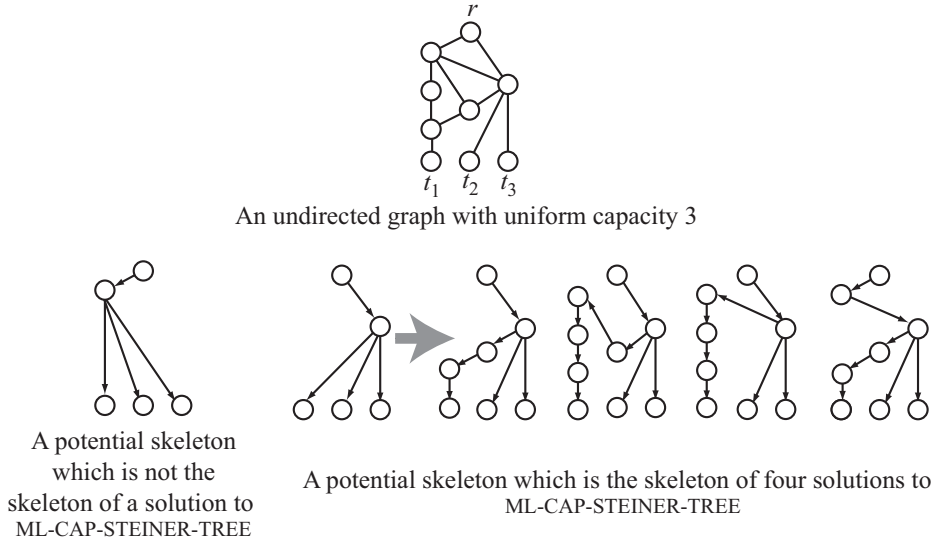
Figure 2: Potential skeletons in a graph G .
