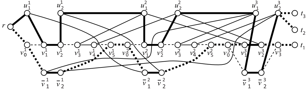
Figure 6: From SAT to CAP-STEINER-TREE.
