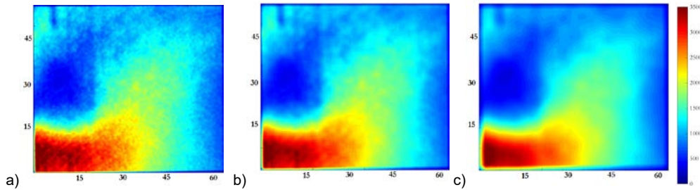
Figure 5. Maps of mean spray density under non-reactive conditions for phase 0^\circ with filter size of a) 25x25 b) 51x51 c) 101x101. Scale in mm
