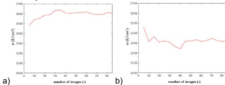
Figure 6. Evolution of the mean density at two different locations in the spray according to the number of processed images for phase 0^\circ
