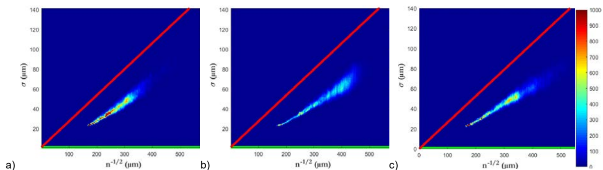
Figure 11. Evolution of the standard deviation of nearest-neighbour inter-droplet distance according to the inverse square-root of mean density for phase at a) 0° b) 135° c) 270°
