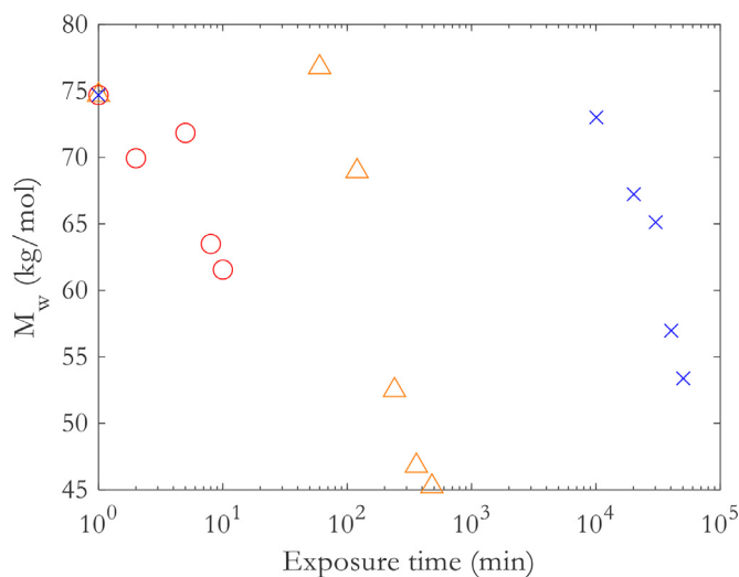
Fig. 7. Average weight molar mass changes for thermal ageing at 210 °C (o), 180 °C (Δ) and hydrolytic ageing at 80 °C (×). Values are given in PMMA equivalent.
