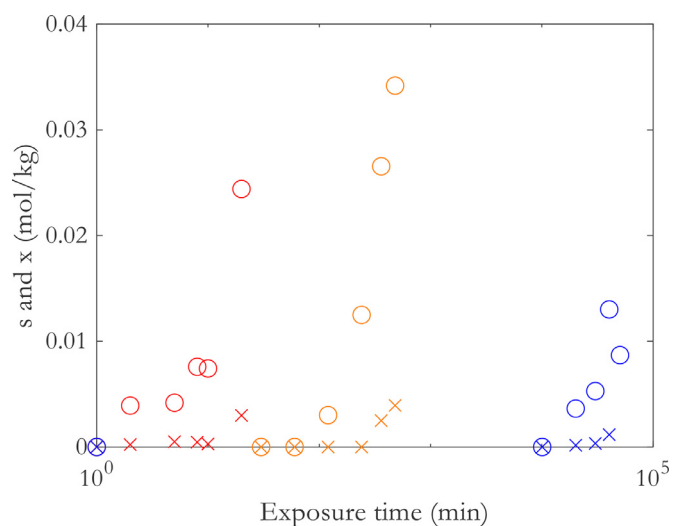
Fig. 10. Chain scission ( \circ ) and crosslinking ( \times ) concentrations after an ageing at 210 °C (red), 180 °C (orange) and hydrolysis at 80 °C (blue).
