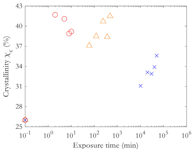
Fig. 4. Crystallinity changes for thermal ageing at 210 °C (o), 180 °C (Δ) and hydrolytic ageing at 80 °C (×).
