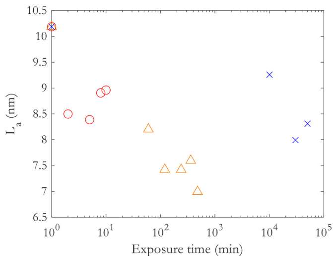
Fig. 5. Changes in thickness of the amorphous layer for thermal ageing at 210 °C (o), 180 °C (Δ) and hydrolytic ageing at 80 °C (×).
