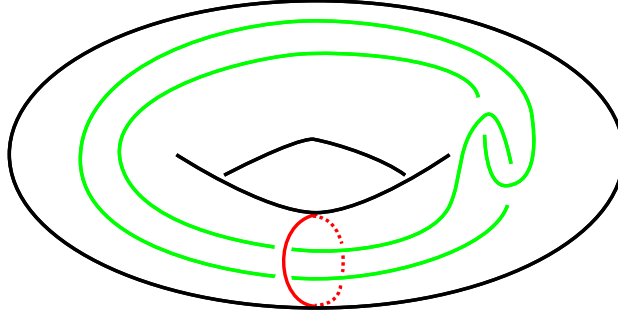
Figure 2. T_2 \subset T_1 .
