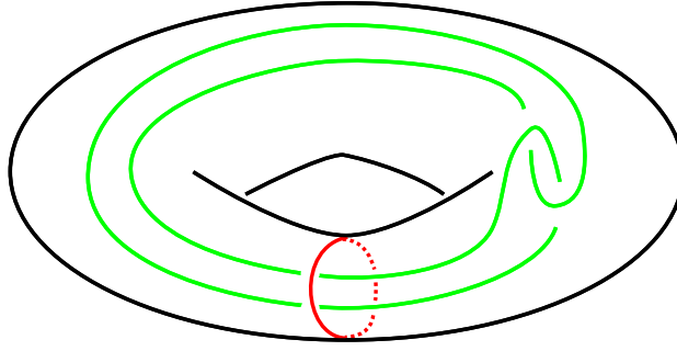
Figure 2. T_2 \subset T_1 .
