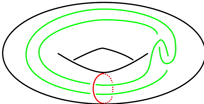
Figure 2.2: T_2 \subset T_1
