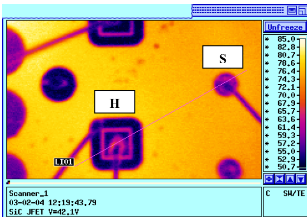
Fig. 4.- IR measurement at low drain bias ( V_{\text{DS}} = 42\text{ V} ) on heating (H) and sensing (S) chips
