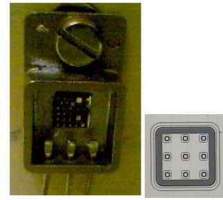
Fig. 3.- Packaged current limiter (metallic TO-220 package). (die de 4\text{ mm} \times 4\text{ mm} ) (limiter 460\mu\text{m} \times 460\mu\text{m} )
