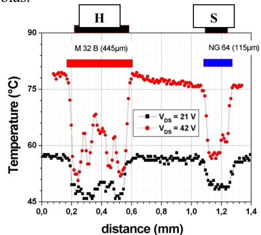
Fig. 5.- Temperature cross-section along LI01 of the left IR-picture (fig. 4).
