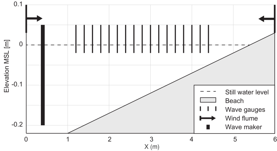
Figure 1: CASH wind-wave flume setup and schematic visualisation.
