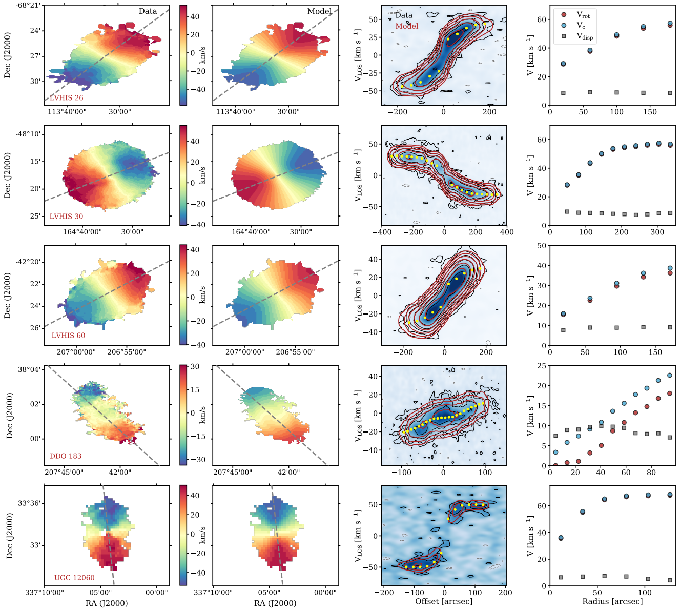
Fig. A.1. Kinematic models of five representative galaxies obtained with 3\text{D} BAROLO. From left to right: (1) observed and (2) best-fitting model velocity field; the dashed grey line shows the average kinematic position angle, while the bar between the two panels show the colour scheme in both velocity fields. (3) Major axis position-velocity diagram: The data is shown in blue, while black contours enclose the data (grey for negative values) and red contours the best-fitting model. The contour levels are at -2, 2, 4, 8, 16, \dots times the mean rms in the corresponding data cube. The recovered rotation velocities are shown in yellow. (4) Rotation velocity (red), circular speed (blue) and velocity dispersion (grey) profiles.
