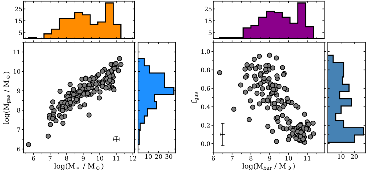
Fig. 1. M_*-M_{\text{gas}} (left) and M_{\text{bar}}-f_{\text{gas}} (right) relation for our sample of galaxies. Typical errorbars are shown in black. The panels at the top and right of each relation show the histograms of the M_* , M_{\text{gas}} , M_{\text{bar}} , and f_{\text{gas}} distributions.
