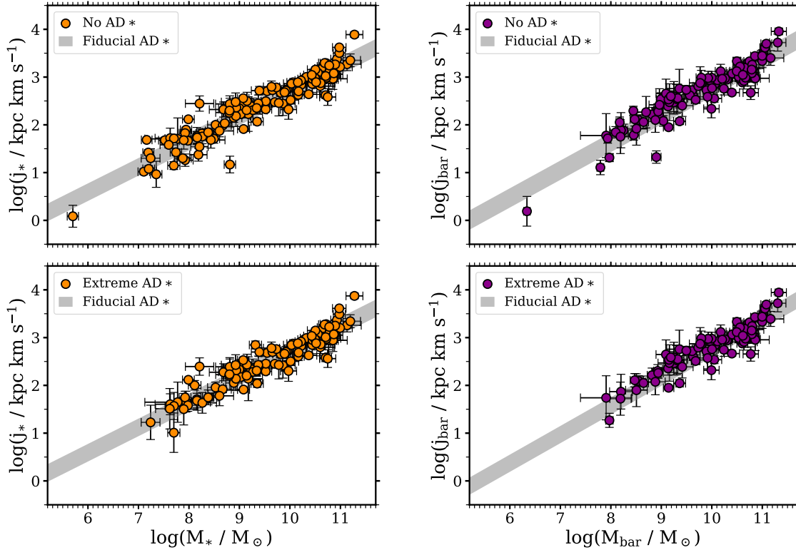
Fig. B.1. Stellar ( left ) and baryonic ( right ) j - M relations under the assumption of none ( top ) or extreme ( bottom ) asymmetric drift correction. In all the panels, the grey band corresponds to the best-fitting relation found for our fiducial correction (see Table 2). Since we applied a convergence criterion, the galaxies are not exactly the same in all the panels.
