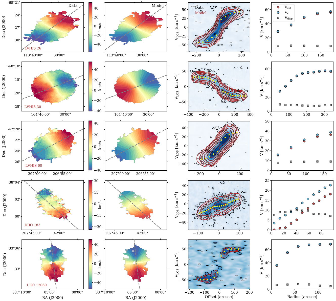
Fig. A.1. Kinematic models of five representative galaxies obtained with 3^{\text{D}} BAROLO. From left to right: (1) observed and (2) best-fitting model velocity field; the dashed grey line shows the average kinematic position angle, while the bar between the two panels show the colour scheme in both velocity fields. (3) Major axis position-velocity diagram: The data is shown in blue, while black contours enclose the data (grey for negative values) and red contours the best-fitting model. The contour levels are at -2, 2, 4, 8, 16, \dots times the mean rms in the corresponding data cube. The recovered rotation velocities are shown in yellow. (4) Rotation velocity (red), circular speed (blue) and velocity dispersion (grey) profiles.
