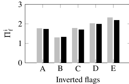
Figure 5: Dimensionless critical flow velocity for the onset of large-amplitude flapping of different inverted flags when sweeping up the flow velocity; \square with and \blacksquare without the rigid splitter plate.
