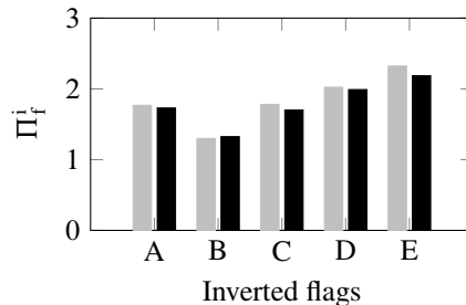
Figure 5: Dimensionless critical flow velocity for the onset of large-amplitude flapping of different inverted flags when sweeping up the flow velocity; (grey) with and (black) without the rigid splitter plate.
