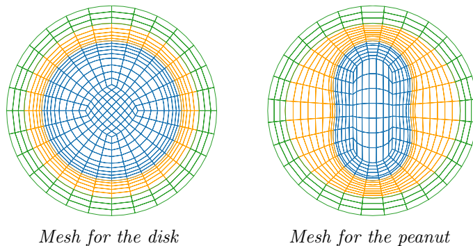
Figure 9. Structured mesh for the circular cavity (left) and the peanut shape cavity (right). The cavity is represented in blue, the exterior domain in orange, and the PML in green. The mesh is locally symmetric along the interface \Gamma . Meshes use quadrangular elements of degree 3, and we use finite elements of degree 8 in the computations (adding degrees of freedom in each element, not represented here).
