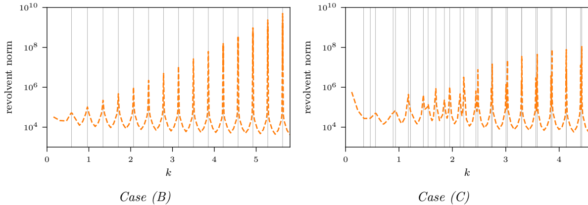
Figure 12. Semi-log plot of the function k \mapsto \|\mathbb{M}_k^{-1}\|_2 in logarithmic scale for the two cases (B) and (C). The vertical grid lines are aligned on the real part of the scattering resonances.
