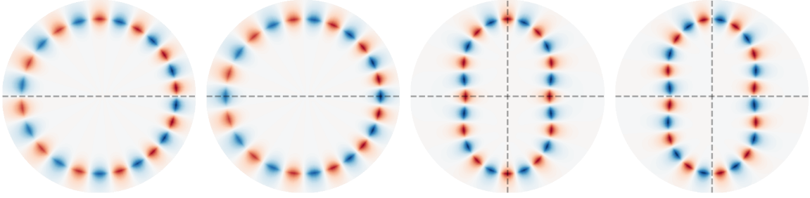
Figure 10. Real part of the 2 resonant modes associated to m = 12 curvilinear oscillations, associated to the resonances in Table 1 : for case (B) (left, middle left), for case (C) (middle right, right). The gray dashed lines represent the symmetry axes of the problem and hence the symmetries of the modes.
