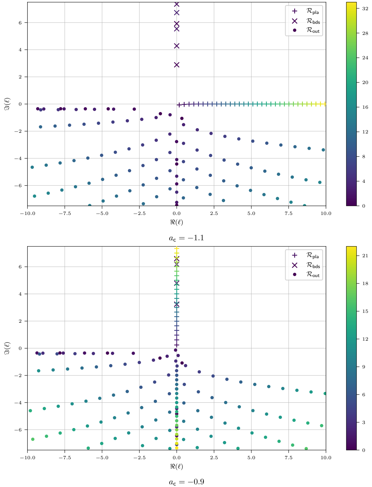
Figure 3. Graph of the sets \mathcal{R}_{33}[-1.1, 1] (top) and \mathcal{R}_{22}[-0.9, 1] (bottom) in the complex plane (\Re(\ell), \Im(\ell)) with \ell \in \mathbb{C} \setminus \mathbb{R}_- . Those sets are computed using complex contour integration [40] on the analytic function Eq. (3.5).
