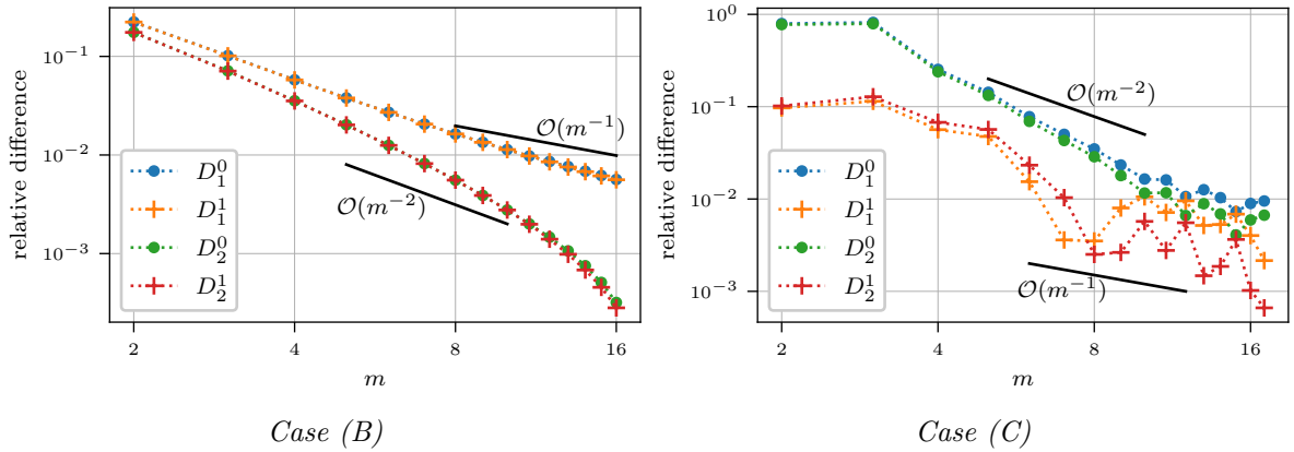
Figure 14. Graphs of the relative difference D_t^s(m) , s = 0, 1 , t = 1, 2 , between the scattering resonances \ell_{\text{fem},m}^s computed via FEM (Step 1), and the asymptotic expansion \sqrt{\lambda_{m,t}^s} via Eq. (4.22), for cases (B) and (C).
