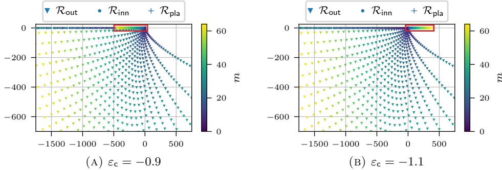
FIGURE 3. Graph of the sets \mathcal{R}_{64}[-0.9, 1] (left) and \mathcal{R}_{64}[-1.1, 1] (right) in the complex plane (\Re(\ell^2), \Im(\ell^2)) , computed using complex contour integration [36] on the analytic function Eq. (3.6).
