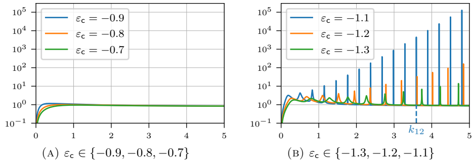
FIGURE 1. Log plot of k \mapsto N_{\epsilon,2}(k) with respect to k for \epsilon_c \in \{-0.9, -0.8, -0.7\} (left), for \epsilon_c \in \{-1.3, -1.2, -1.1\} (right). The value k_{12} marked on the graphs corresponds to the reference value used in Figure 2.
