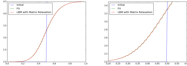
Fig. 1 Viscous Shock Test with \epsilon = 0.1 : Comparison of the viscous profiles of the finite volume and the lattice Boltzmann scheme.
