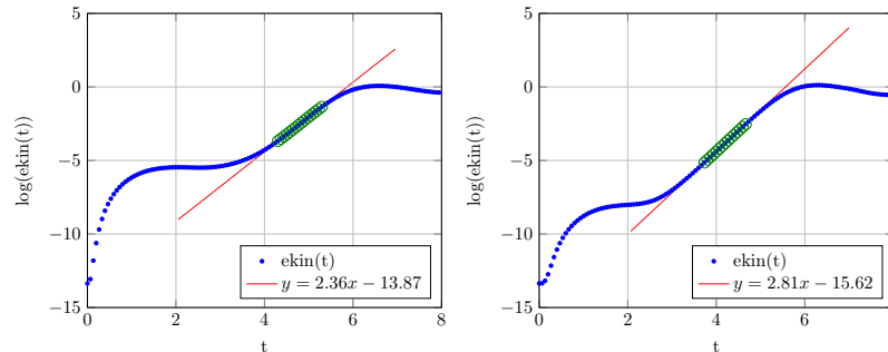
Fig. 11 Growth of the kinetic energy during the simulation. Measures that have been accounted for the linear regression are identified with green marks and the regression line is in red. Results for grid sizes Nx \times Ny = 512 \times 512 and Nx \times Ny = 2048 \times 2048 .
