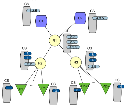
(b) Aggregation based inter-domain routing.
