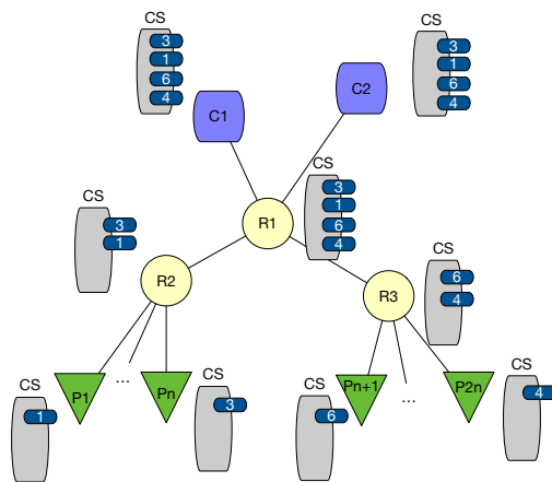
(a) Conventional flat NDN.
