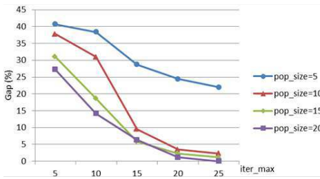
Fig. 2: Effects of pop_{size} and iter_{max} on solution quality
