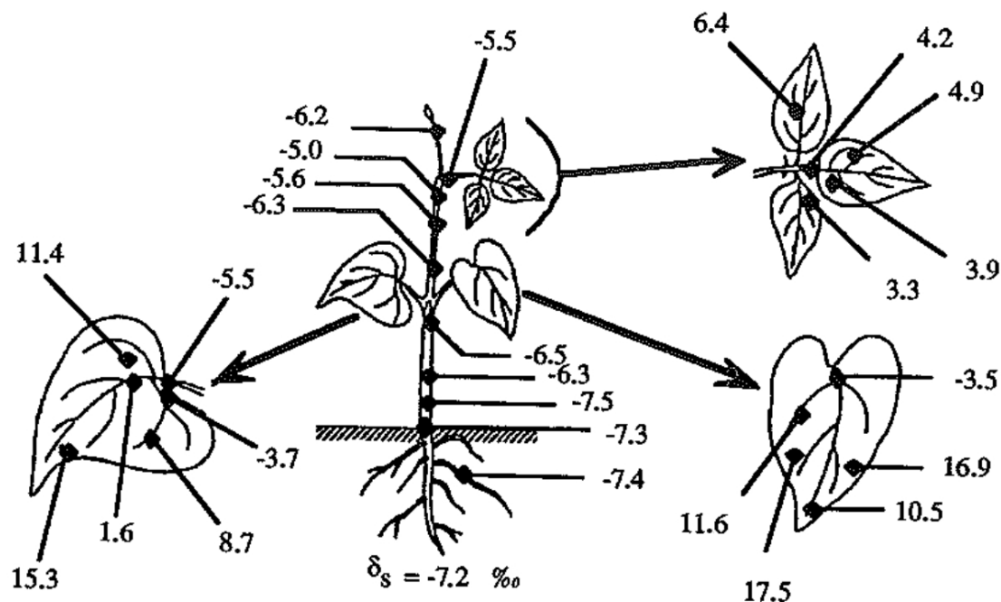
Figure 12. Evolution of the water oxygen content in the different organs of a bean plant. The isotopic composition of water of hydroponics is -7.2 \text{ ‰} (Bariac et al. , 1994a).
