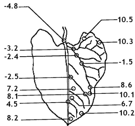
Figure 6. Mapping the water oxygen content in a primary leaf taken from a bean plant (Bariac et al. , 1994a). The ^{18}\text{O} content of irrigation water was -7.2\% .
