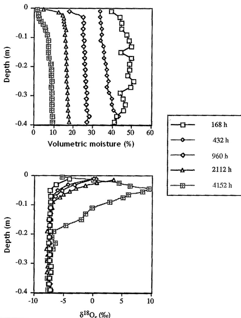
Figure 8. Change with time of the isotopic profile ( \delta^{18}O ) of water inside soil columns submitted to evaporation and without water supply. Note: Profiles were previously homogenized for water and heavy isotopes contents (Boujamloui, 1993).
