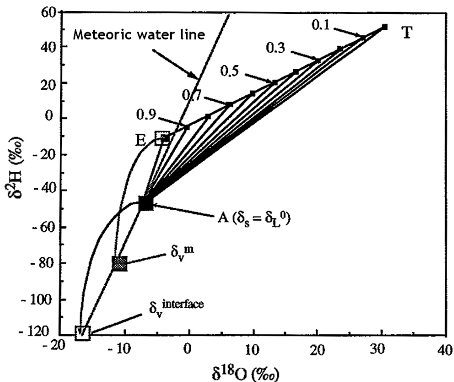
Figure 11. Meteoric water line and transpiration lines in a \delta^2\text{H} - \delta^{18}\text{O} diagram
