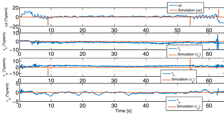
FIGURE 16 Control signal for the suboptimal nonlinear control with a trajectory tracking task, for outdoor flight [Colour figure can be viewed at wileyonlinelibrary.com ]
