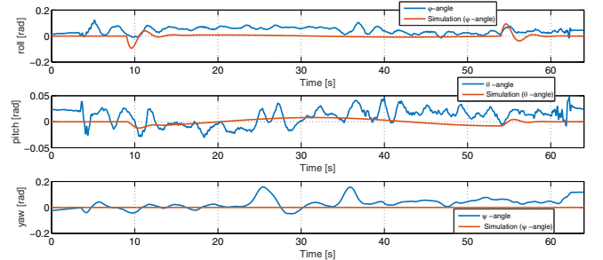
(B) Orientation of the vehicle
