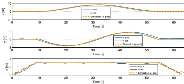
(A) Position of the vehicle
