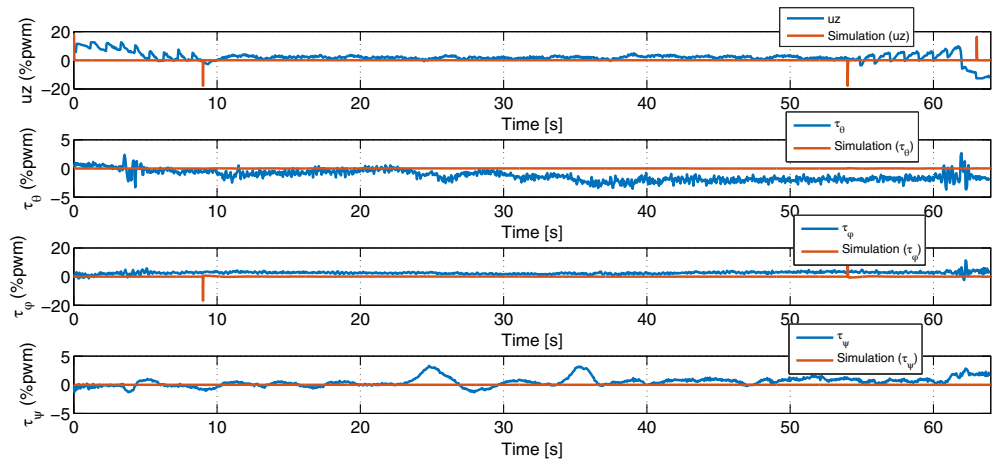
FIGURE 20 Control signal for the PD controllers with a trajectory tracking task, for outdoor flight [Colour figure can be viewed at wileyonlinelibrary.com ]
