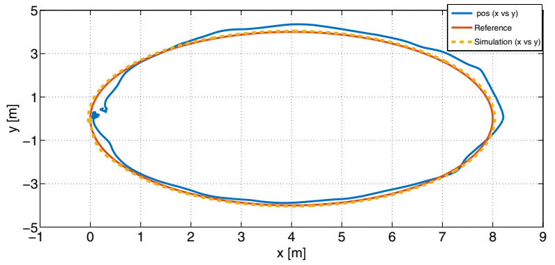
FIGURE 19 Position of the vehicle using PD controllers with a trajectory tracking task, for outdoor flight [Colour figure can be viewed at wileyonlinelibrary.com ]
