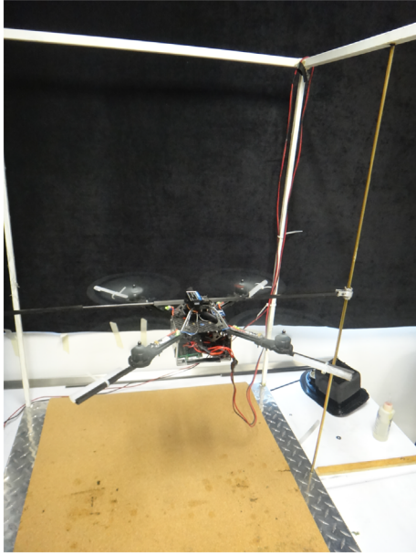
FIGURE 2 Quadrotor experimental setup of 4DOF [Colour figure can be viewed at wileyonlinelibrary.com ]
