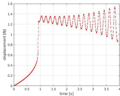
(a) Beam element free vibration
