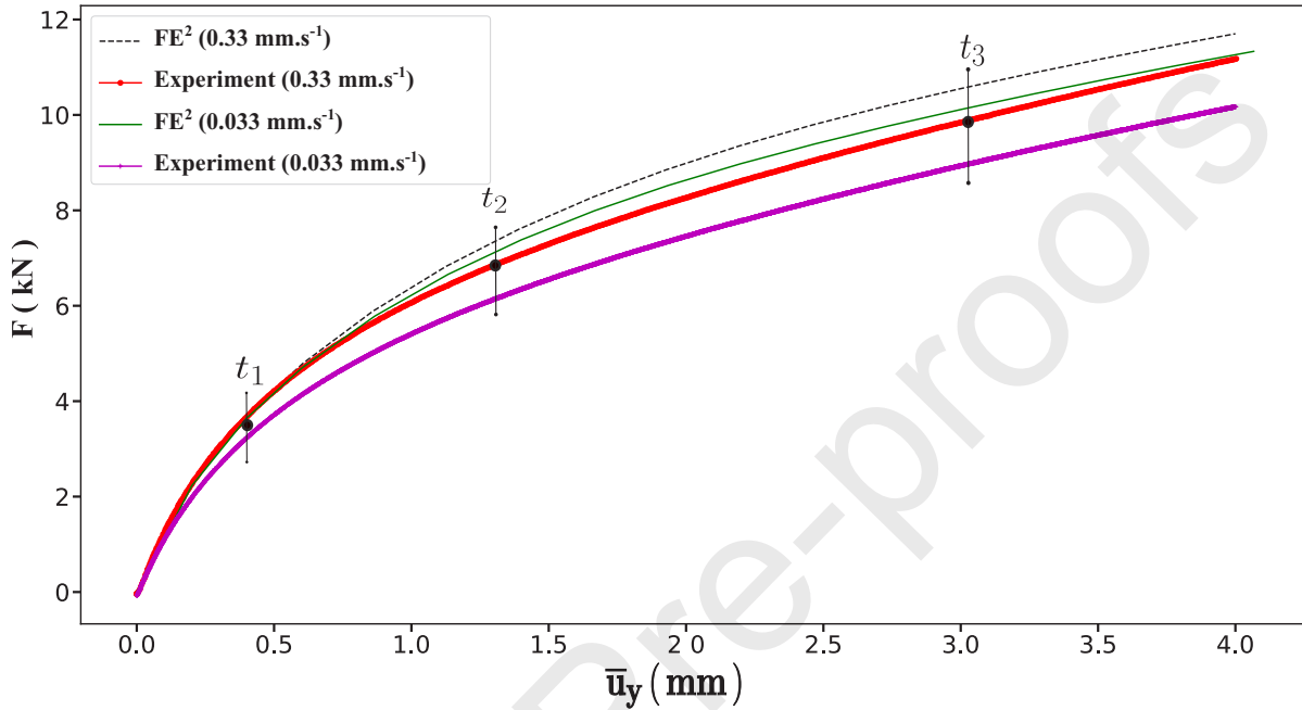
Figure 13: Macroscopic responses of the studied composite for the \pm 45 stacking sequence under both loading rates 0.033 and 0.33 mm.s -1 . Comparison between DIC and FE 2 approaches.
