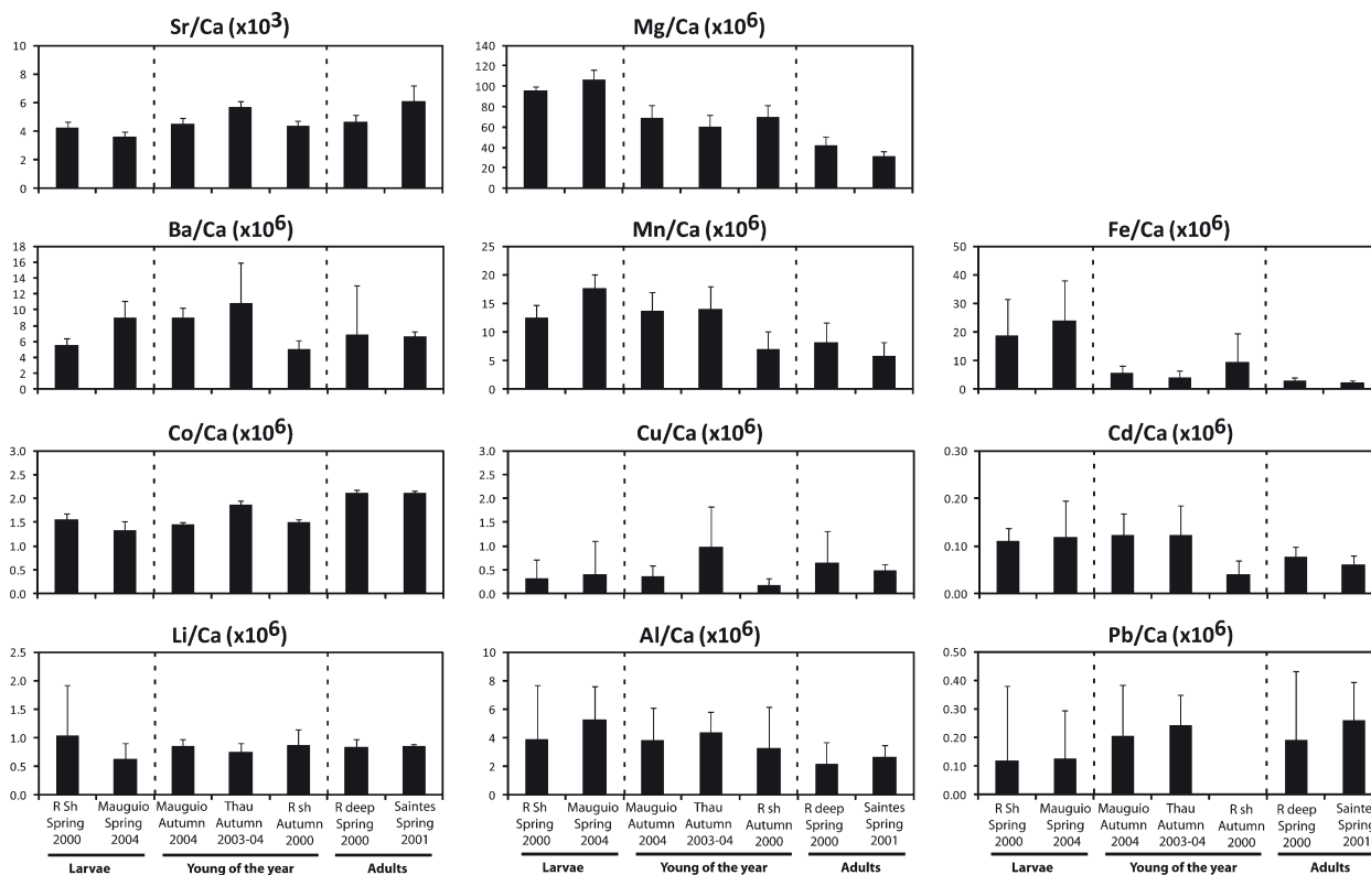
Fig. 2. – Mean ( \pm sd) of elemental ratios by site (R Sh, Rhône shallow; R deep, Rhône deep). Both years in Thau coastal lagoon are grouped. Life stages are mentioned below the graphics.
