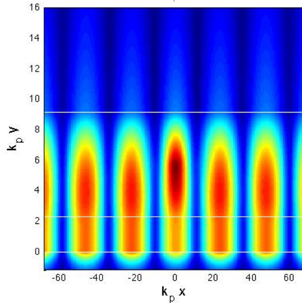
Figure 10. Local density of states for a source located in the middle of the dielectric waveguide. The wavelength is \lambda = 1550\text{nm} and the regime is that of strong coupling.
