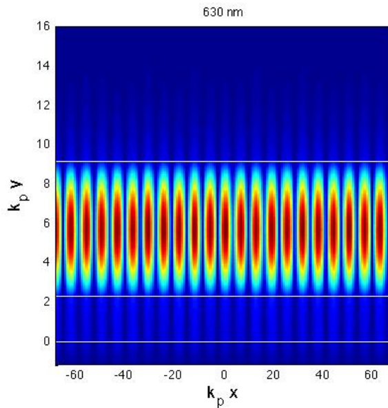
Figure 9. Local density of states for a source located in the middle of the dielectric waveguide. The wavelength is \lambda = 630\text{nm} and the regime is that of strong coupling.
