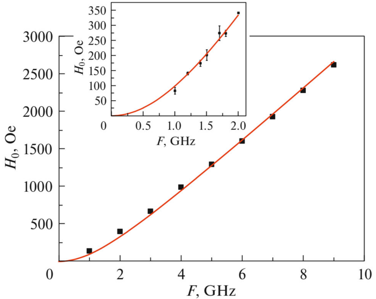
Fig. 3. Frequency dependence of resonance field H_0 for YIG in the TCFC/YIG heterostructure with a 40-nm-thick TCFC film. The solid line shows the dependence (1) for a magnetization of M_0 \approx 100 G. Inset: frequency dependence of H_0 in the low-frequency range. The error shown corresponds to the frequency dependence of the difference between the resonance fields of two lines with the highest intensities.
