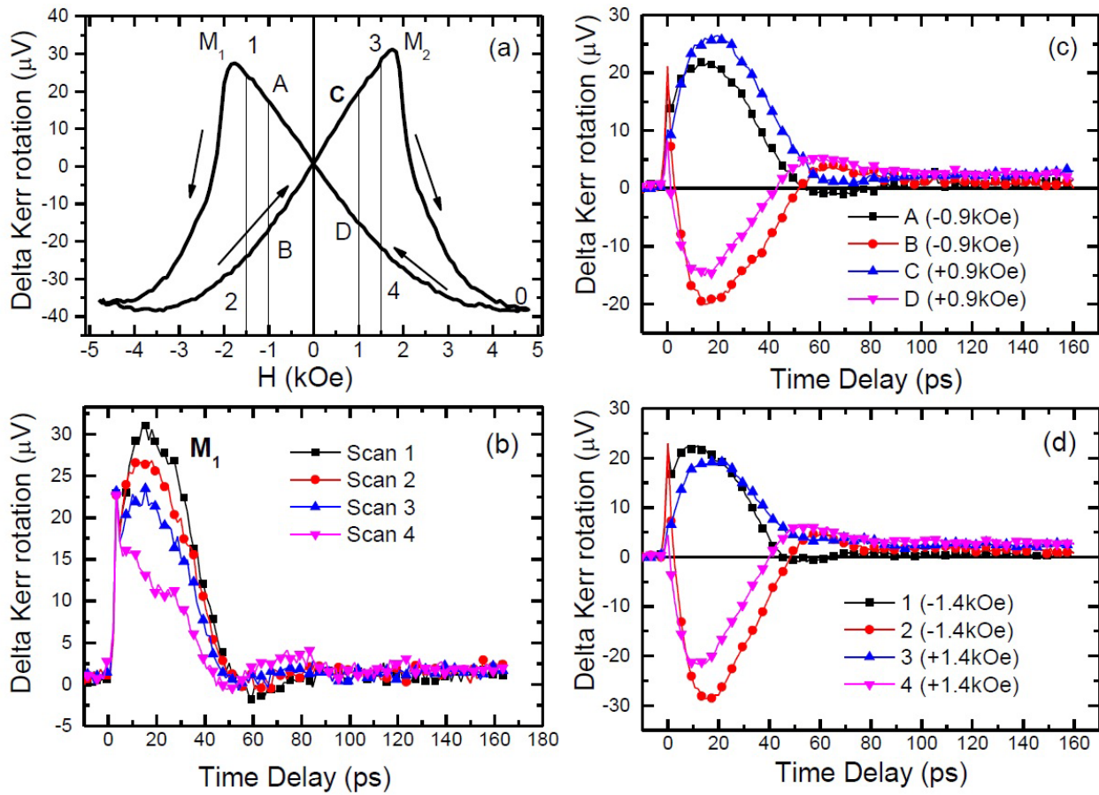
Figure 3. ‘Hard axis’ geometry. (a) Kerr rotation hysteresis loops at maximum of the first oscillation ( t = 20 ps); dependences of the Kerr rotation on the delay time for different points on the Kerr hysteresis loop shown in the picture (a); instability in point M_1 is illustrated by consecutive identical scans (b); data measured in points A, B, C, D (c) and in points 1, 2, 3, 4 (d).
