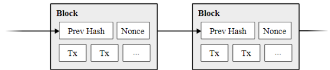
Fig. 1. The architecture of blockchain
