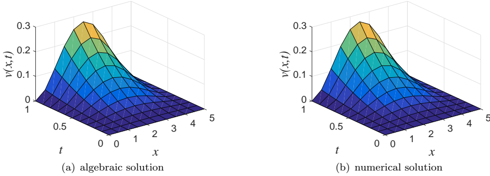
Figure 3: The comparison of the numerical and algebraic solutions at different matching point when n = 5 .
