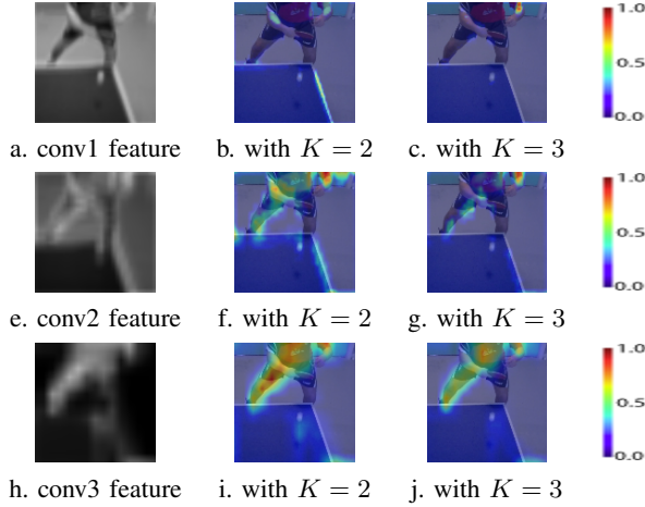
Fig. 4. Visualization with features from different conv layers and Influence of K - value in thresholding. At top row, result with first conv layer features. At middle row, second conv layer features and at the third row, results with third conv layer features
