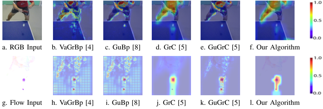
Fig. 3. Different Visualization algorithm outputs of our model for the class: Defensive Backhand block. First row shows the visualization for RGB input data and second row does the same for Flow input data.
