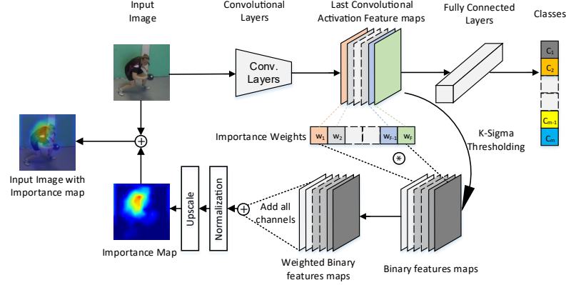
Fig. 2. Overview of proposed visualization algorithm. Features are extracted from the last convolutional layer after the activation function (upper part). Binary features maps are generated. Importance weights are calculated. Importance map is computed as a normalized linear combination with channel weights and visualized as a heat-map on the original image
