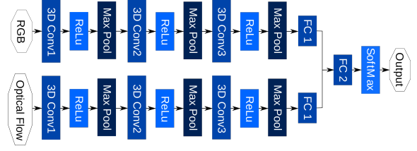
Fig. 1. Analyzed TSTCNN architecture.
