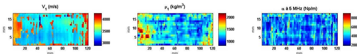
Figure 5. C-scan results
