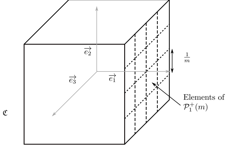
Figure 5 – Splitting the face \mathfrak{C}_1^+ into m^{d-1} hyperrectangles
