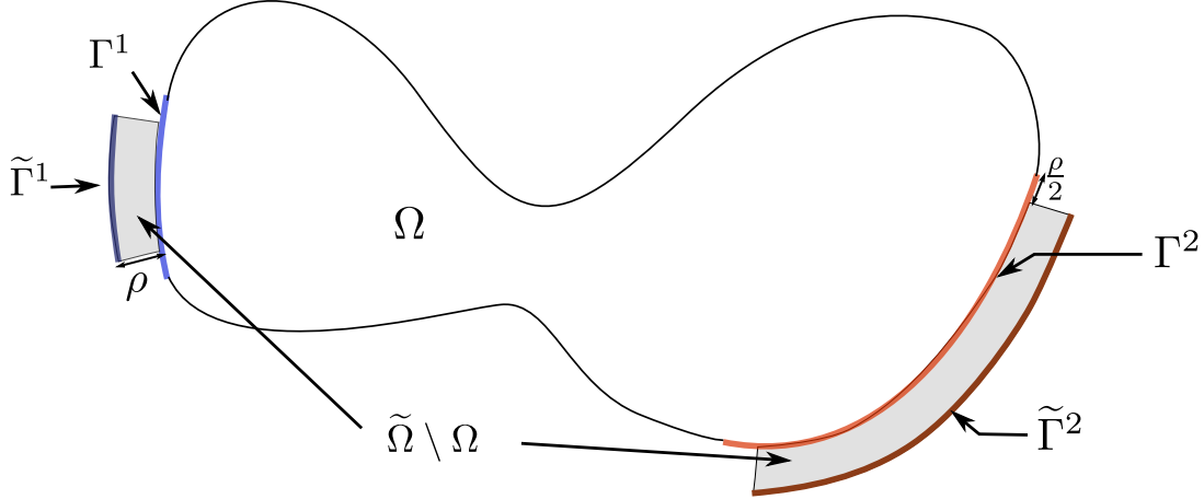
Figure 11 – Example of possible (\tilde{\Omega}, \tilde{\Gamma}^1, \tilde{\Gamma}^2)
