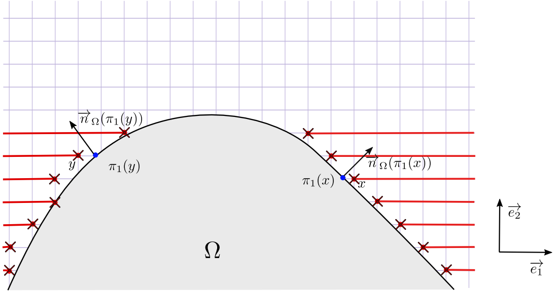
Figure 13 – The crosses correspond to points in \Gamma_n^1 . By sake of clarity we only represent how we prolongate the stream in the direction \vec{e}_1 (represented by the bold lines). Note that in the figure, \vec{n}_{\Omega}(\pi_1(x)) \cdot \vec{e}_1 > 0 and \vec{n}_{\Omega}(\pi_1(y)) \cdot \vec{e}_1 < 0 . The corresponding p is chosen big enough.
