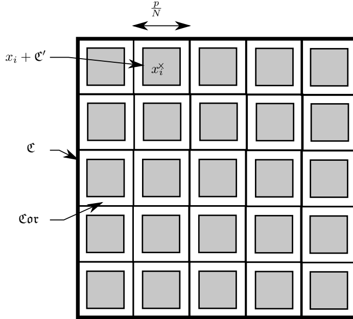
Figure 7 – Paving \mathfrak{C} with translates of \mathfrak{C}'
