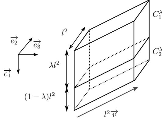
Figure 9 – Representation of C^\lambda ( d = 3 )
