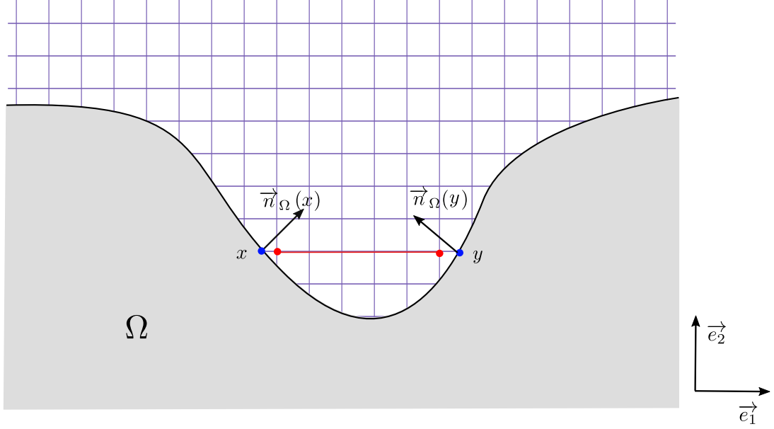
Figure 15 – Illustration of the case where there exists e such that \|\tilde{f}_n(e)\|_2 > M .
