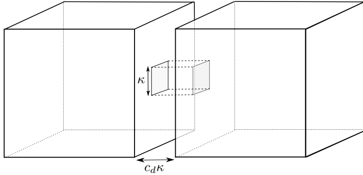
Figure 2 – Connecting streams in cubes at mesoscopic level
