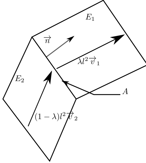
Figure 10 – Representation of the set E ( d = 2 )
