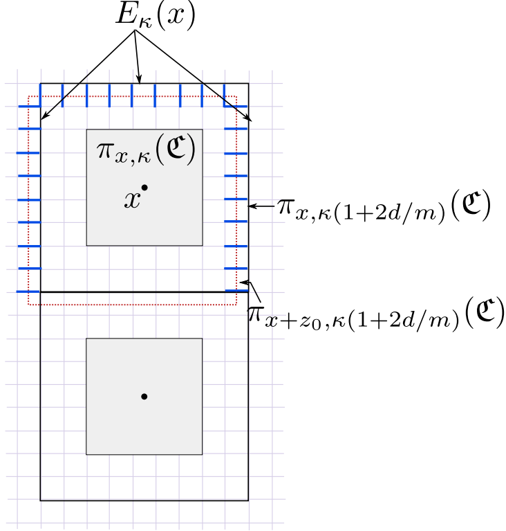
Figure 12 – Choice of z_0 . The edges in bold represent edges where we will affect the value given by \vec{\sigma}_p^{disc} .
