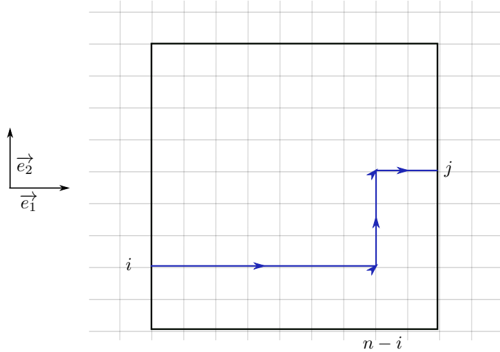
Figure 3 – The path associated with \gamma_{i,j} for j > i
