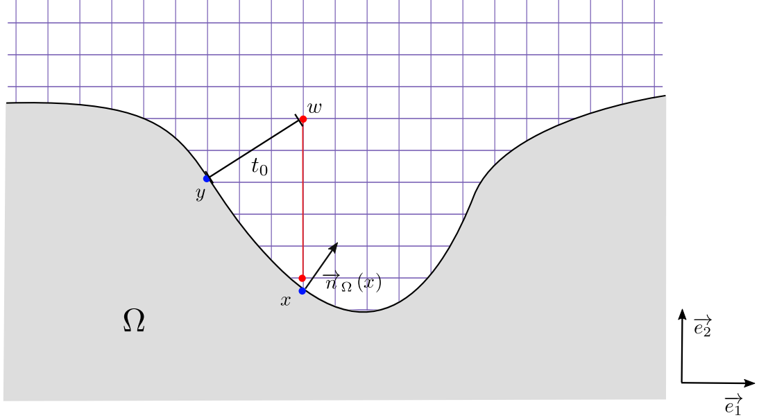
Figure 16 – Illustration of the case where the node law is not respected in \mathcal{V}_2(\Omega, r_0/2p) .
