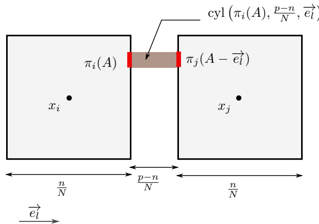
Figure 8 – Connecting streams in two adjacent cubes at mesoscopic level
