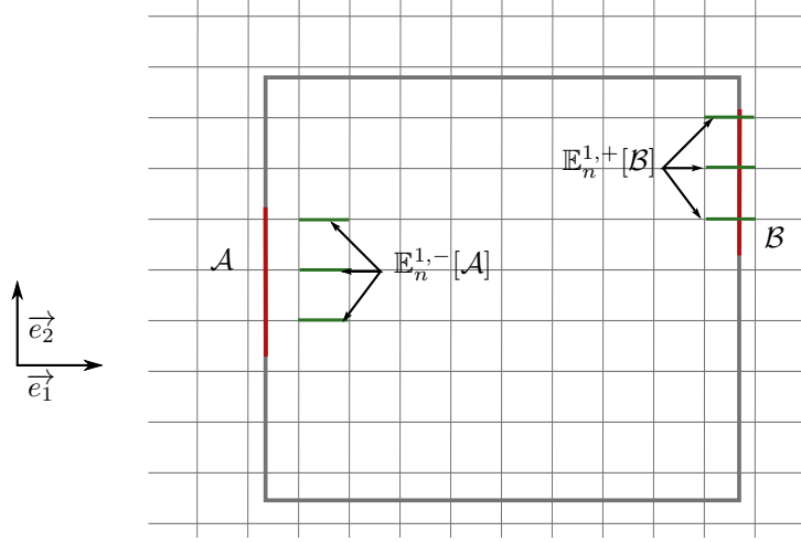
Figure 4 – The sets \mathbb{E}_n^{1,-}[\mathcal{A}] and \mathbb{E}_n^{1,+}[\mathcal{B}]
