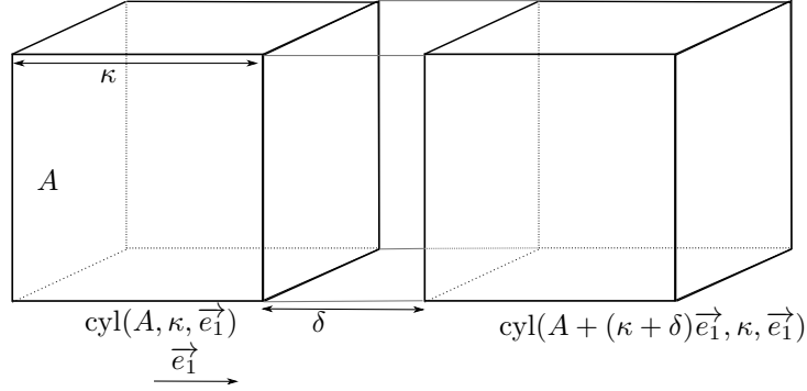
Figure 1 – Connecting two streams in a cylinder
