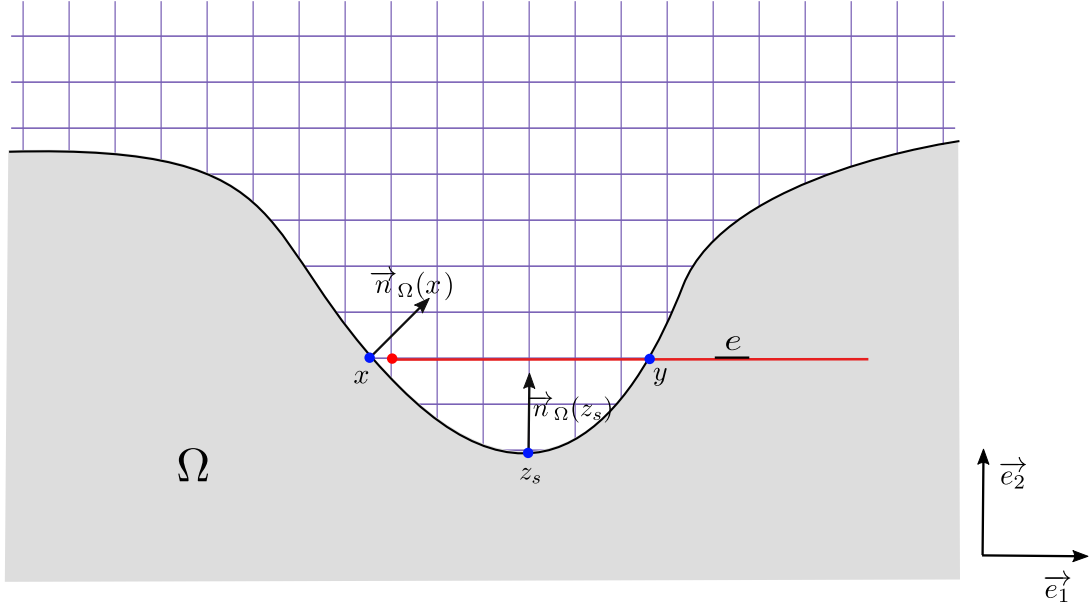
Figure 14 – Illustration of the case where there exists e with its two endpoints in \Omega_n in the support of \tilde{f}_n^{(p)} - f_n^{(p)} .
