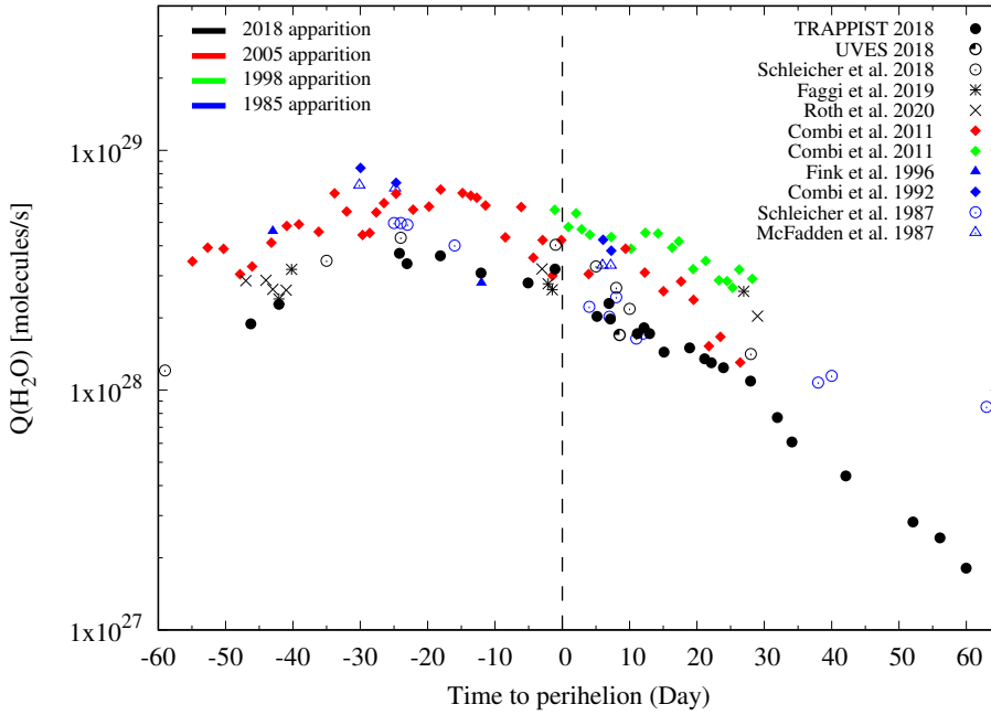
Fig. 2. H 2 O production rates of comet 21P as a function of days to perihelion in 2018 compared to the previous apparitions (1985, 1998, and 2005). The data are described in more detail in Sect. 3.2.
