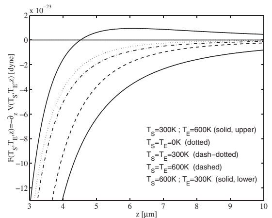
FIG. 2. Surface-atom force F^{\text{neq}}(z) calculated from Eq. (9), for different thermal configurations.
