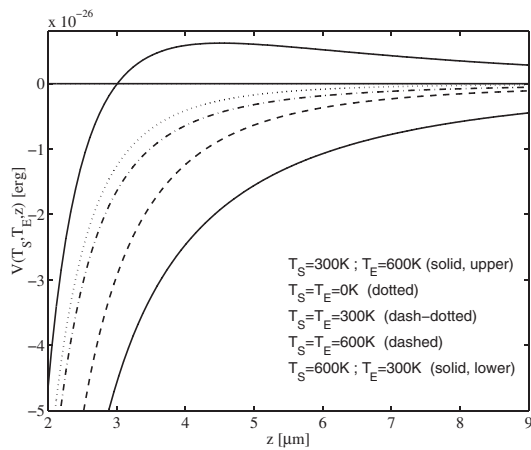
FIG. 1. Surface-atom potential energy V^{\text{neq}}(z) = -\int_z^{+\infty} dz' F^{\text{neq}}(z') calculated from Eq. (9), for different thermal configurations.
